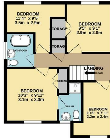
1ST FLOOR 482 sq.ft. (44.8 sq.m.) approx.
