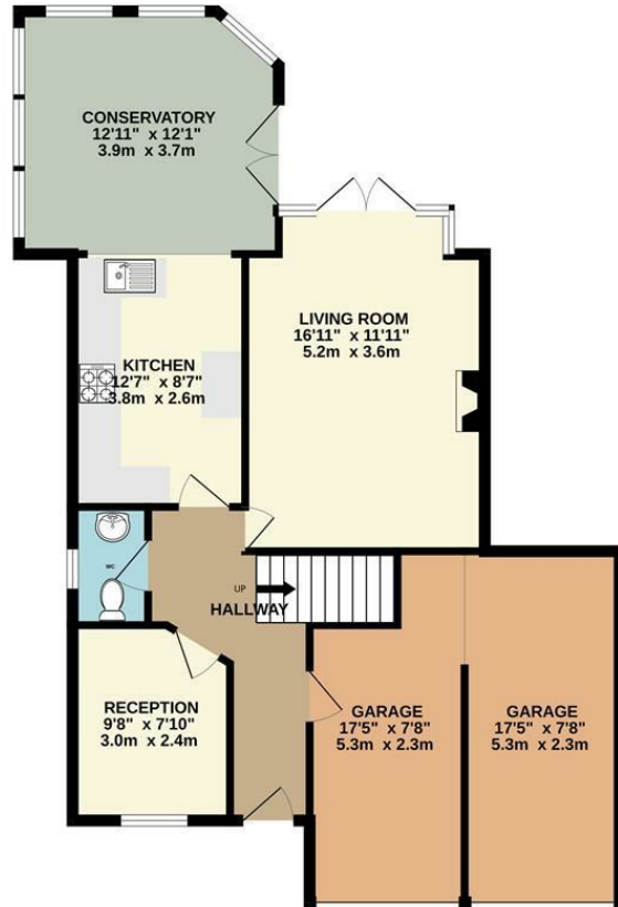
GROUND FLOOR 892 sq.ft. (82.9 sq.m.) approx.
